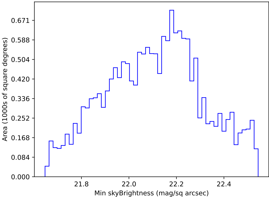
early_u_fpextra3.0_v3.4_10yrs WFD u band: Min skyBrightness
