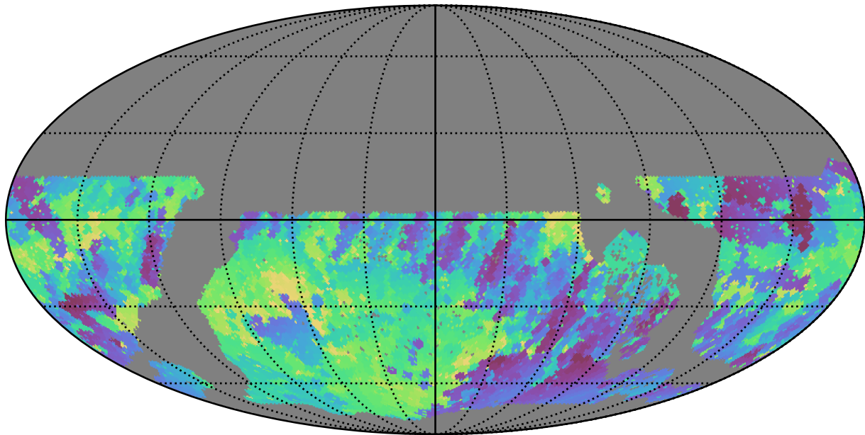
early_u_fpextra3.0_v3.4_10yrs WFD r band: Min skyBrightness
