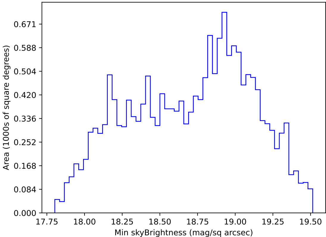
early_u_fpextra3.0_v3.4_10yrs WFD r band: Min skyBrightness
