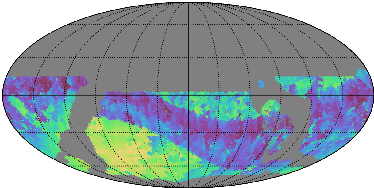
early_u_fpextra3.0_v3.4_10yrs WFD i band: Min skyBrightness
