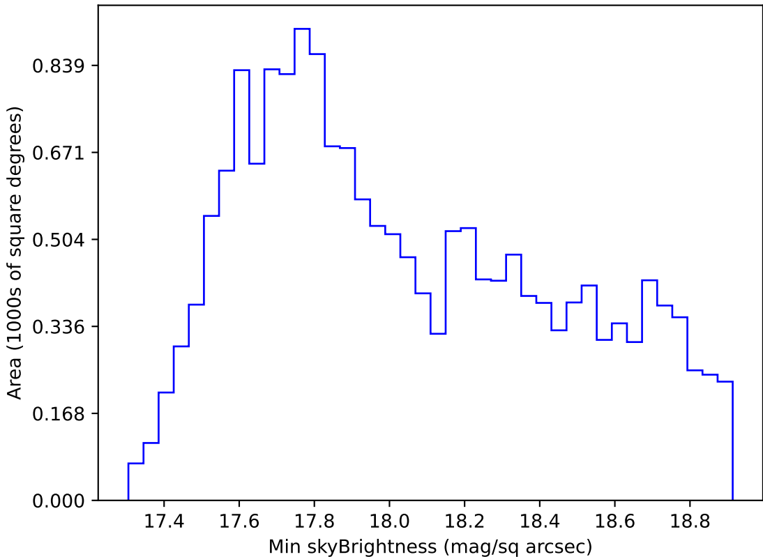
early_u_fpextra3.0_v3.4_10yrs WFD i band: Min skyBrightness
