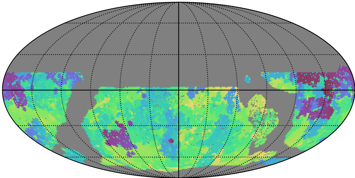
early_u_fpextra3.0_v3.4_10yrs WFD g band: Min skyBrightness
