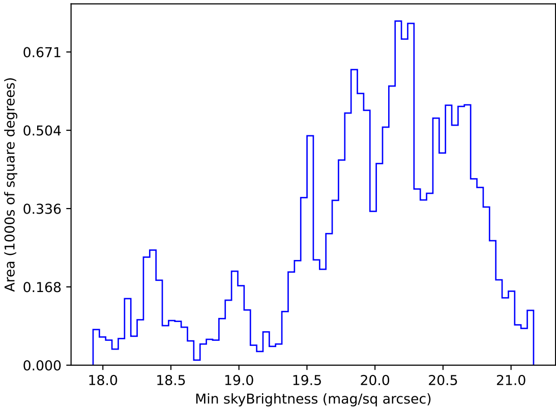
early_u_fpextra3.0_v3.4_10yrs WFD g band: Min skyBrightness
