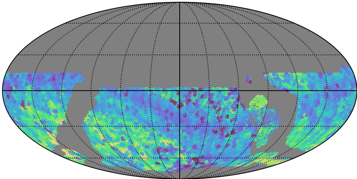
early_u_fpextra3.0_v3.4_10yrs WFD all bands: Min skyBrightness
