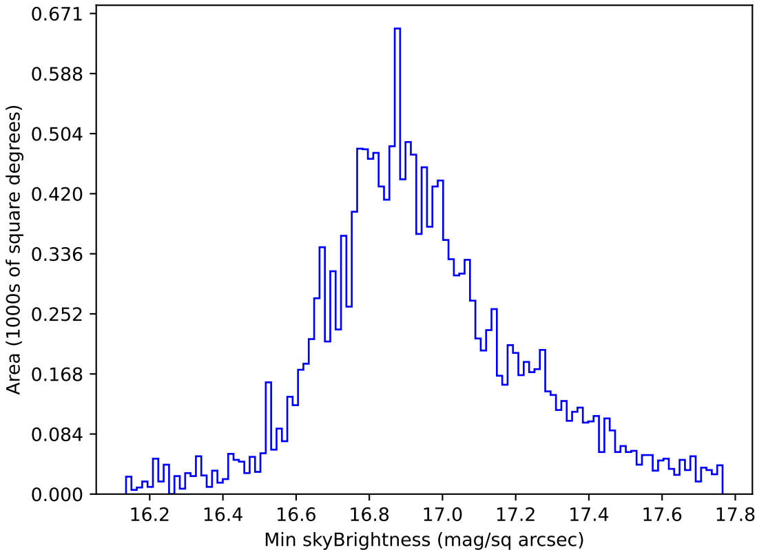
early_u_fpextra3.0_v3.4_10yrs WFD all bands: Min skyBrightness
