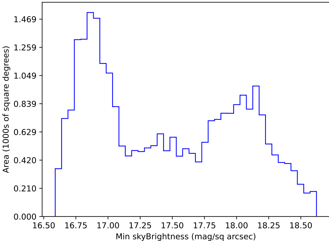
early_u_fpextra3.0_v3.4_10yrs All sky z band: Min skyBrightness
