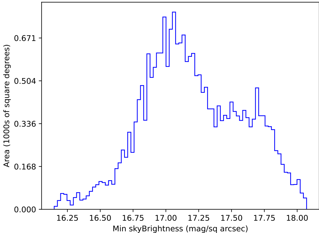
early_u_fpextra3.0_v3.4_10yrs All sky y band: Min skyBrightness
