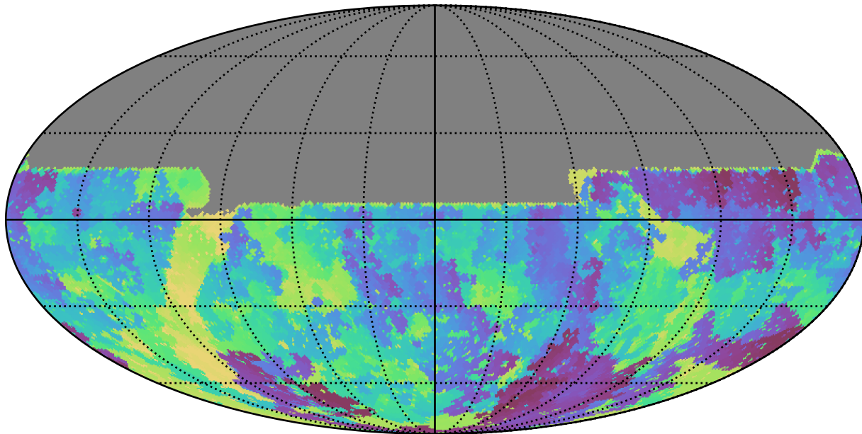
early_u_fpextra3.0_v3.4_10yrs All sky u band: Min skyBrightness
