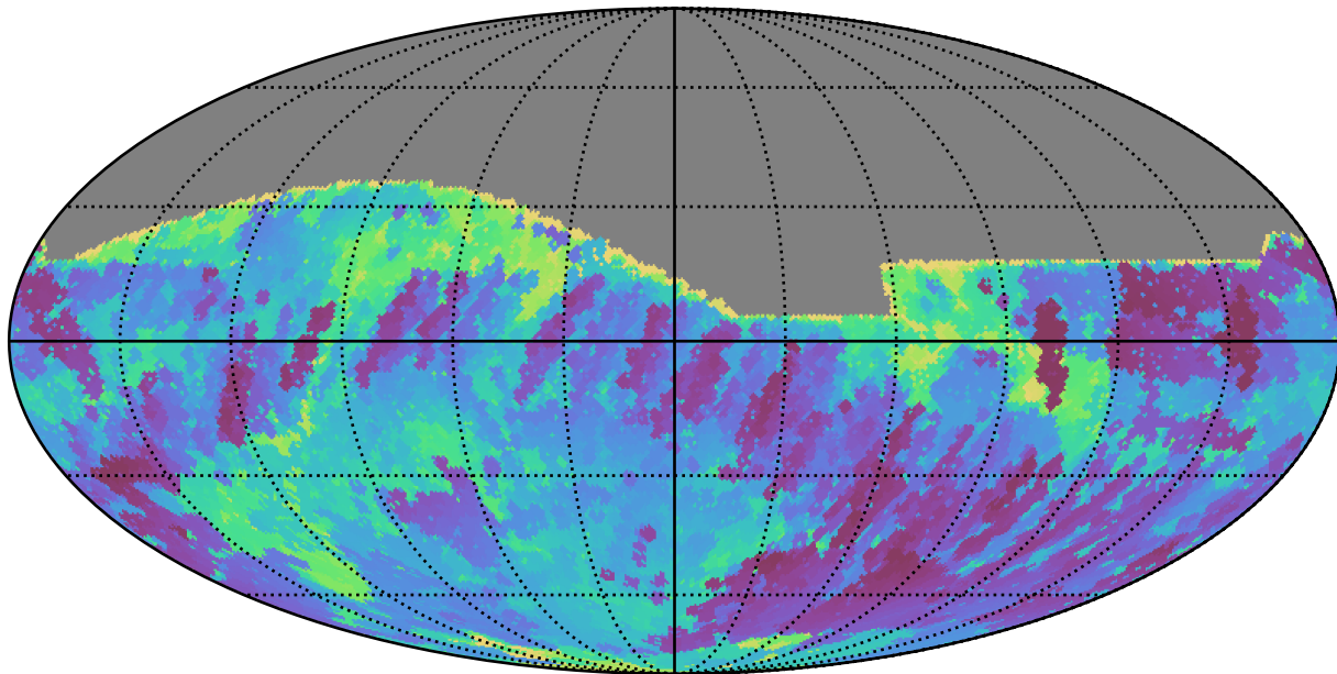
early_u_fpextra3.0_v3.4_10yrs All sky r band: Min skyBrightness
