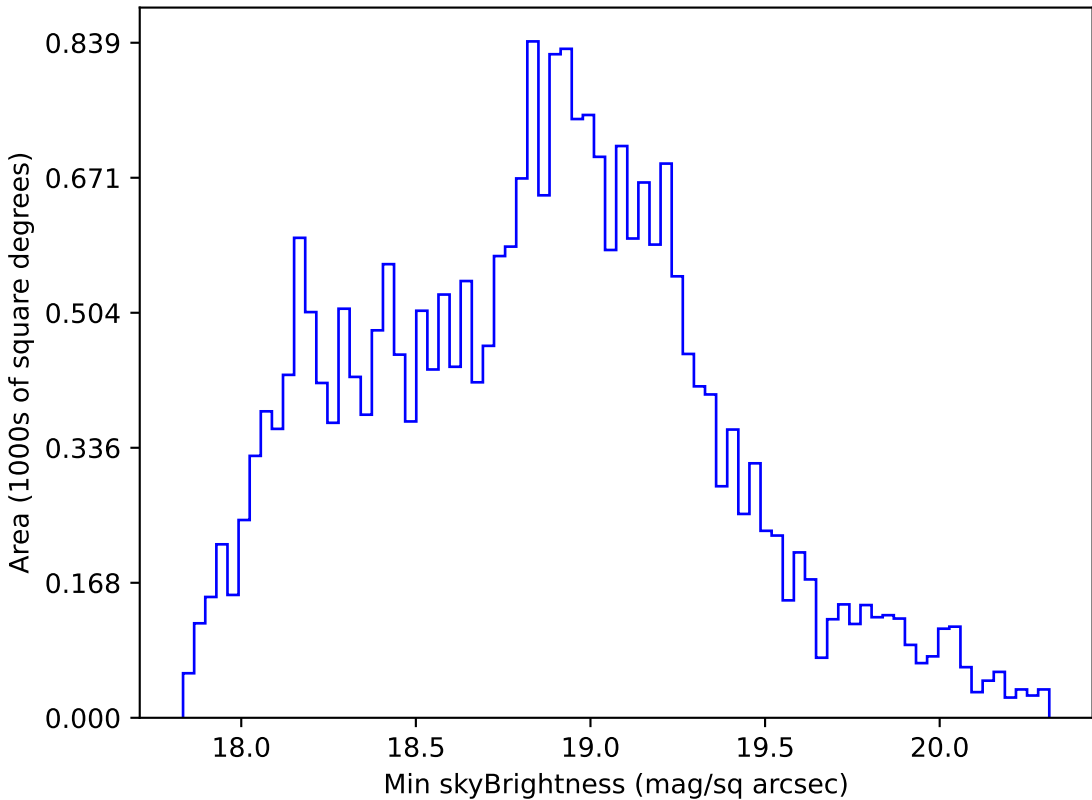
early_u_fpextra3.0_v3.4_10yrs All sky r band: Min skyBrightness
