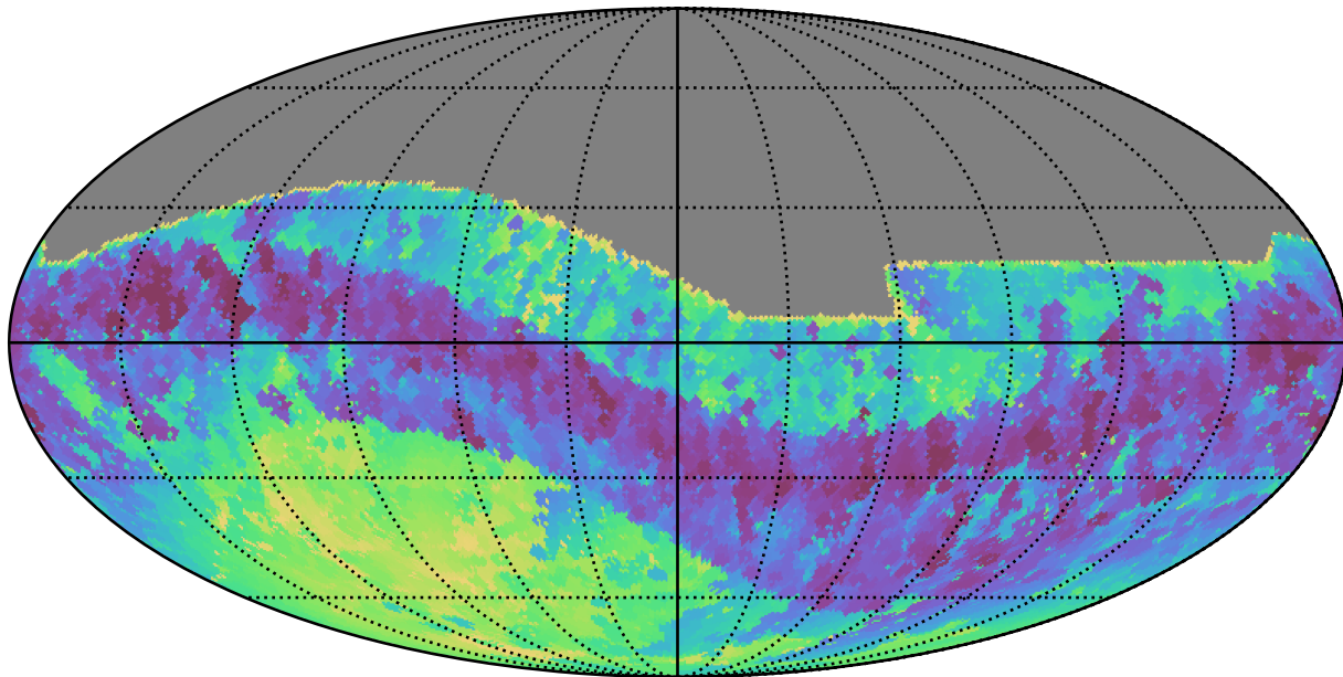
early_u_fpextra3.0_v3.4_10yrs All sky i band: Min skyBrightness
