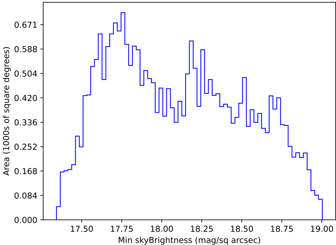
early_u_fpextra3.0_v3.4_10yrs All sky i band: Min skyBrightness
