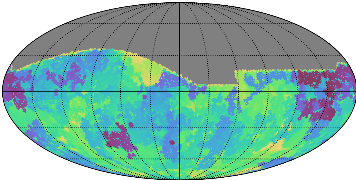
early_u_fpextra3.0_v3.4_10yrs All sky g band: Min skyBrightness
