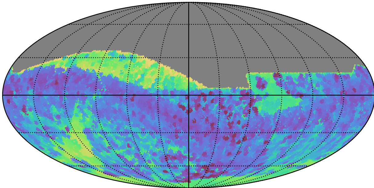
early_u_fpextra3.0_v3.4_10yrs All sky all bands: Min skyBrightness
