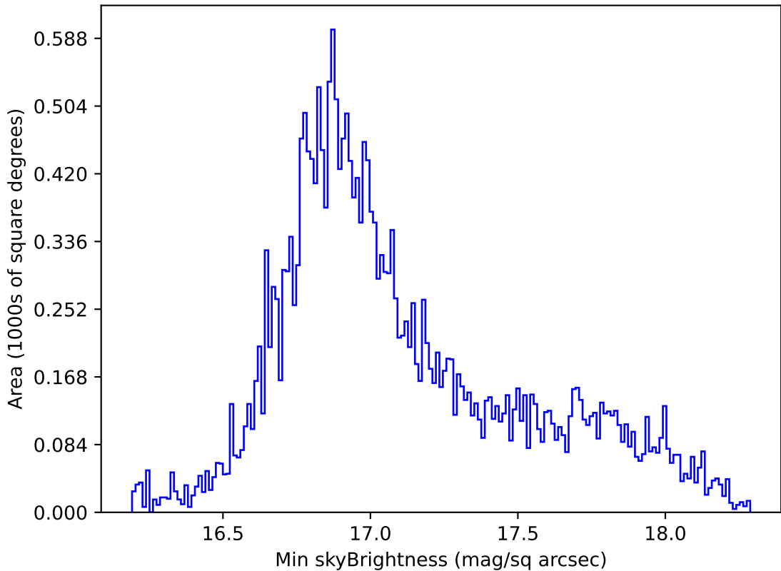
early_u_fpextra3.0_v3.4_10yrs All sky all bands: Min skyBrightness
