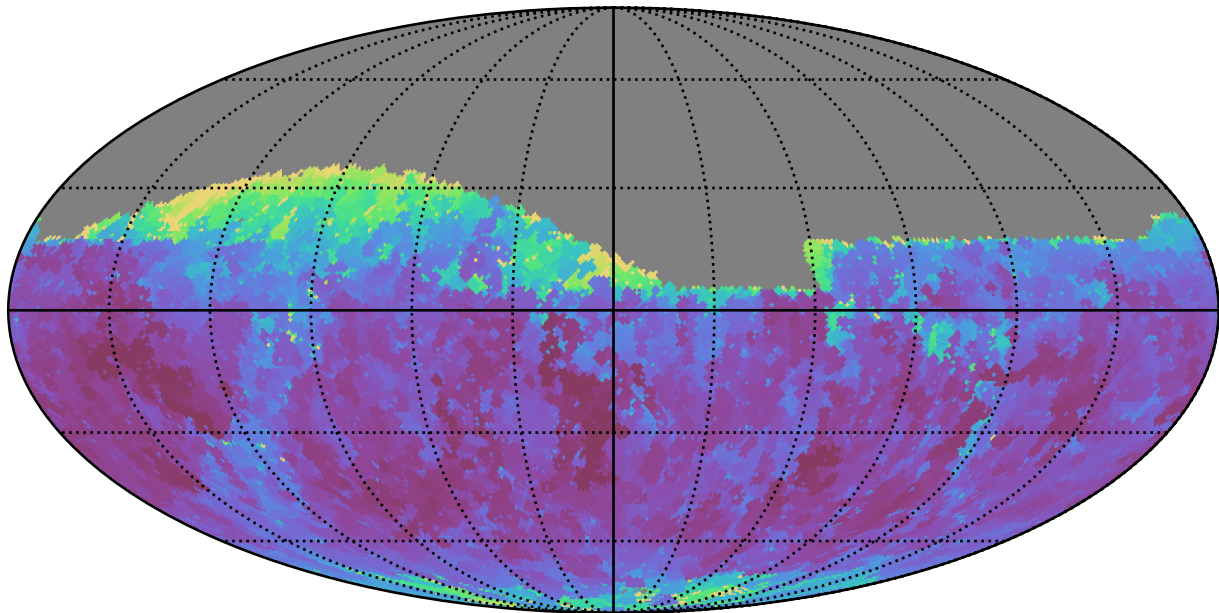
early_u_fpextra3.0_v3.4_10yrs Yr 1 z band: Min seeingGeom
