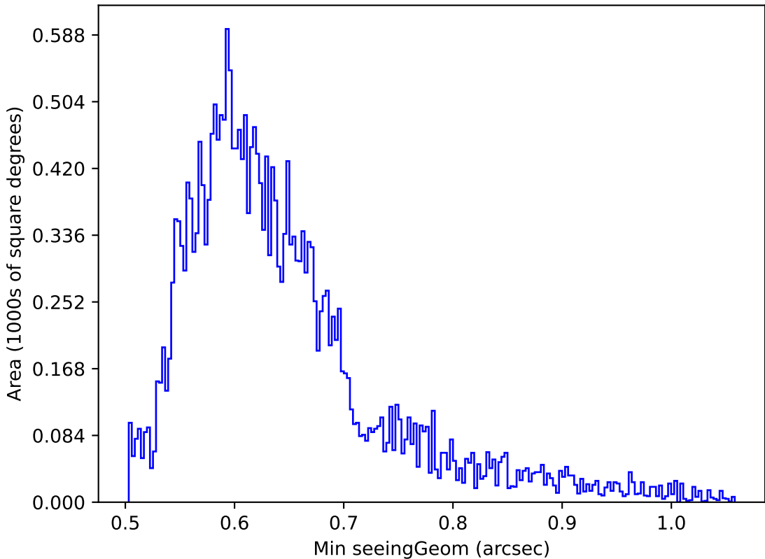
early_u_fpextra3.0_v3.4_10yrs Yr 1 z band: Min seeingGeom
