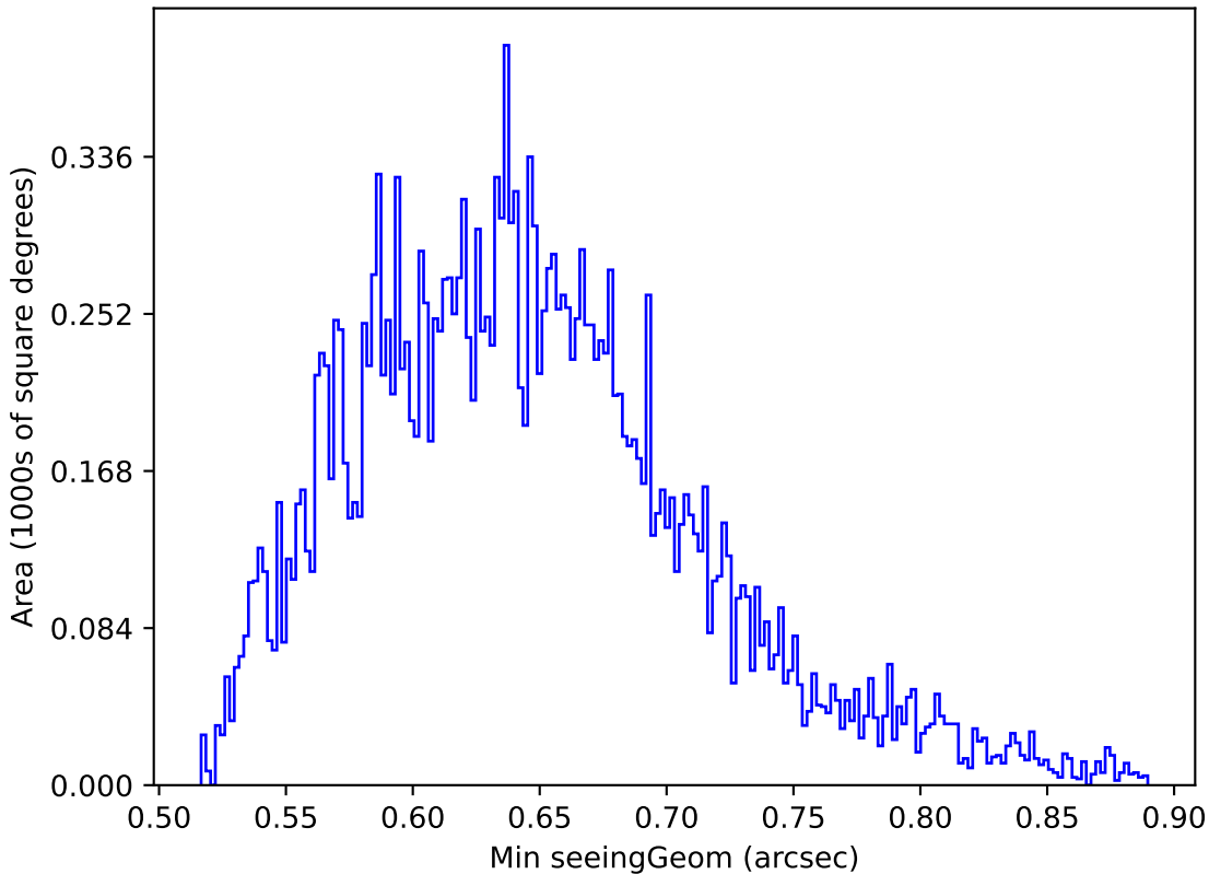
early_u_fpextra3.0_v3.4_10yrs Yr 1 y band: Min seeingGeom
