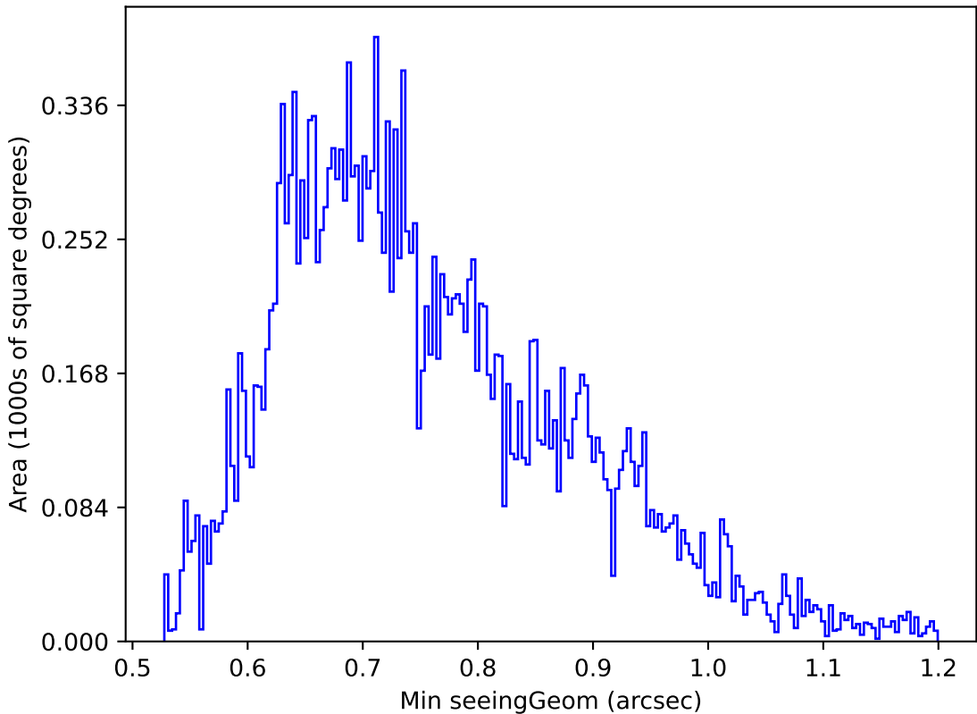
early_u_fpextra3.0_v3.4_10yrs Yr 1 u band: Min seeingGeom
