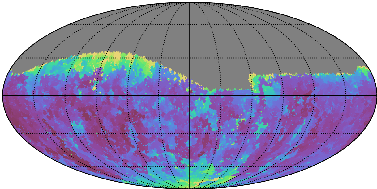
early_u_fpextra3.0_v3.4_10yrs Yr 1 g band: Min seeingGeom
