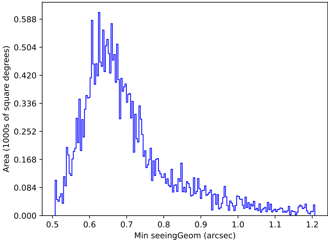
early_u_fpextra3.0_v3.4_10yrs Yr 1 g band: Min seeingGeom
