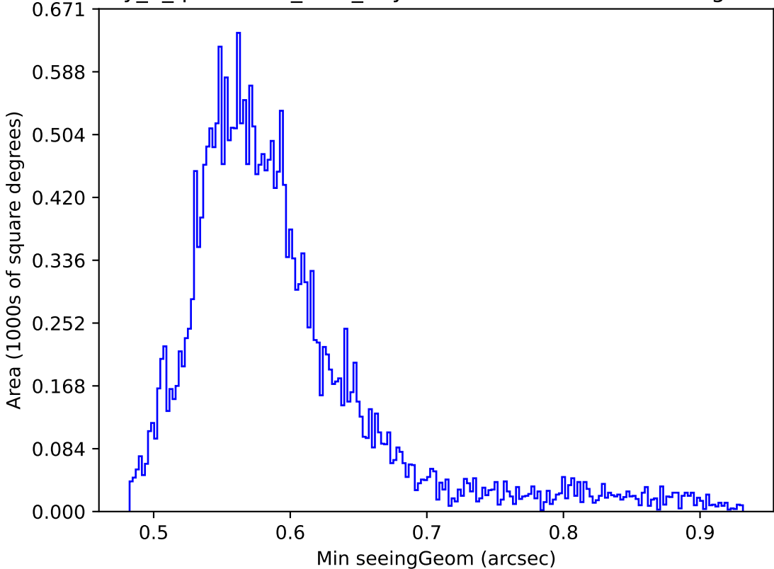
early_u_fpextra3.0_v3.4_10yrs Yr 1 all bands: Min seeingGeom
