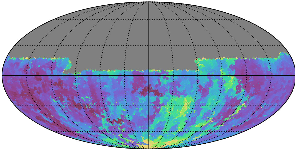
early_u_fpextra3.0_v3.4_10yrs Yr 1 u band: Min seeingEff
