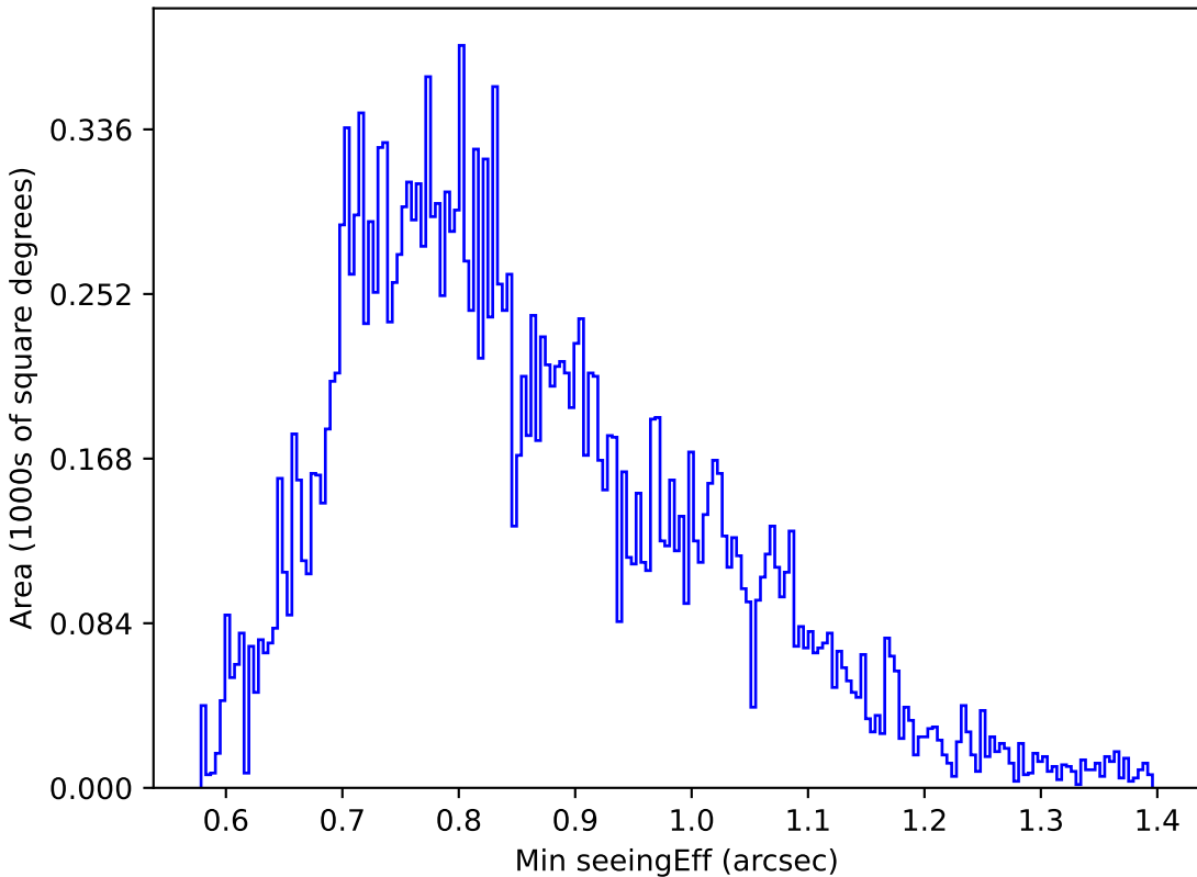
early_u_fpextra3.0_v3.4_10yrs Yr 1 u band: Min seeingEff
