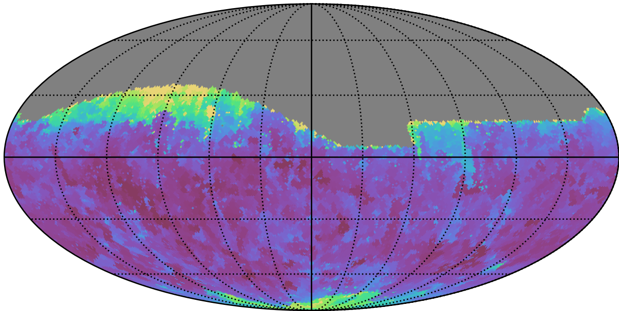
early_u_fpextra3.0_v3.4_10yrs Yr 1 r band: Min seeingEff
