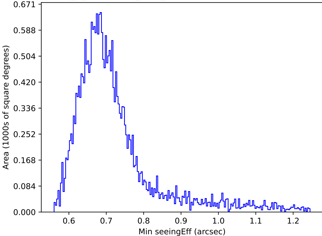
early_u_fpextra3.0_v3.4_10yrs Yr 1 r band: Min seeingEff
