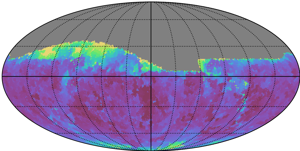
early_u_fpextra3.0_v3.4_10yrs Yr 1 i band: Min seeingEff
