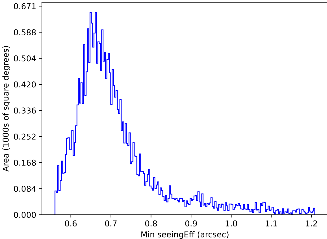
early_u_fpextra3.0_v3.4_10yrs Yr 1 i band: Min seeingEff
