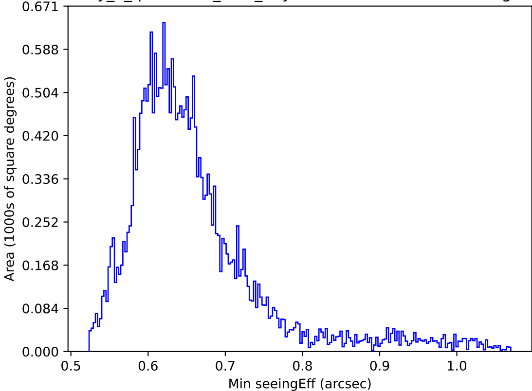
early_u_fpextra3.0_v3.4_10yrs Yr 1 all bands: Min seeingEff
