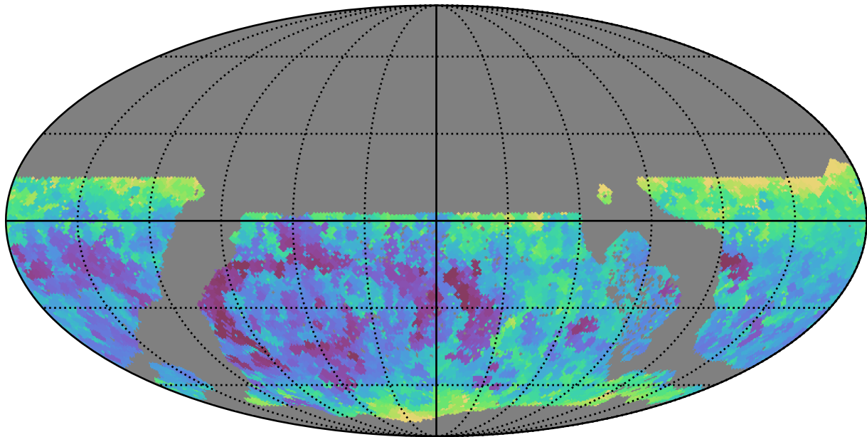
early_u_fpextra3.0_v3.4_10yrs WFD z band: Min seeingEff
