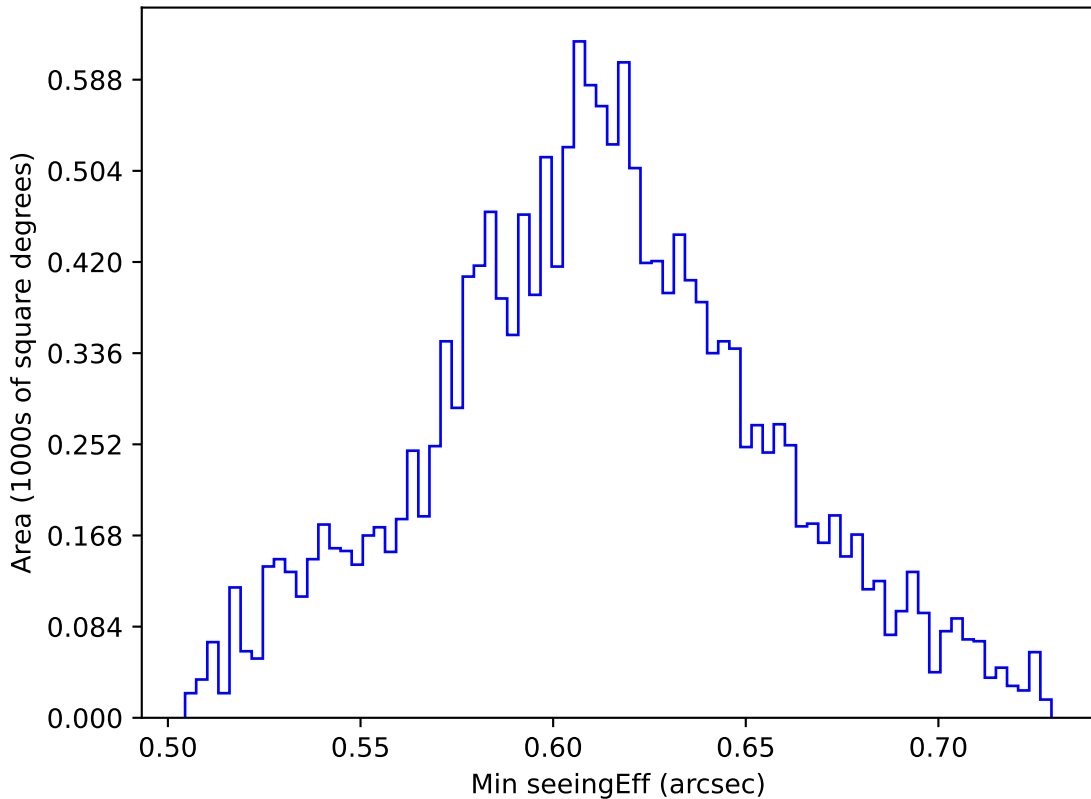
early_u_fpextra3.0_v3.4_10yrs WFD z band: Min seeingEff
