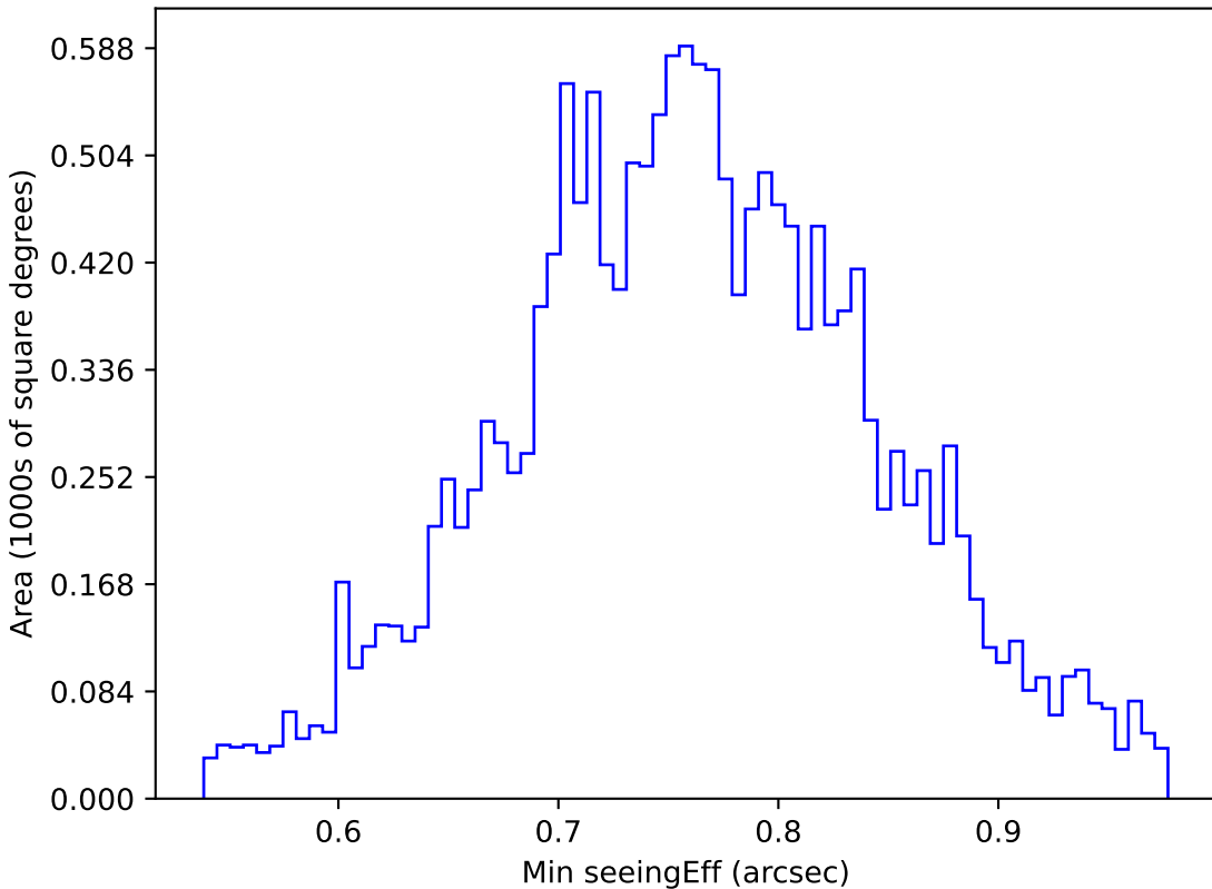
early_u_fpextra3.0_v3.4_10yrs WFD u band: Min seeingEff
