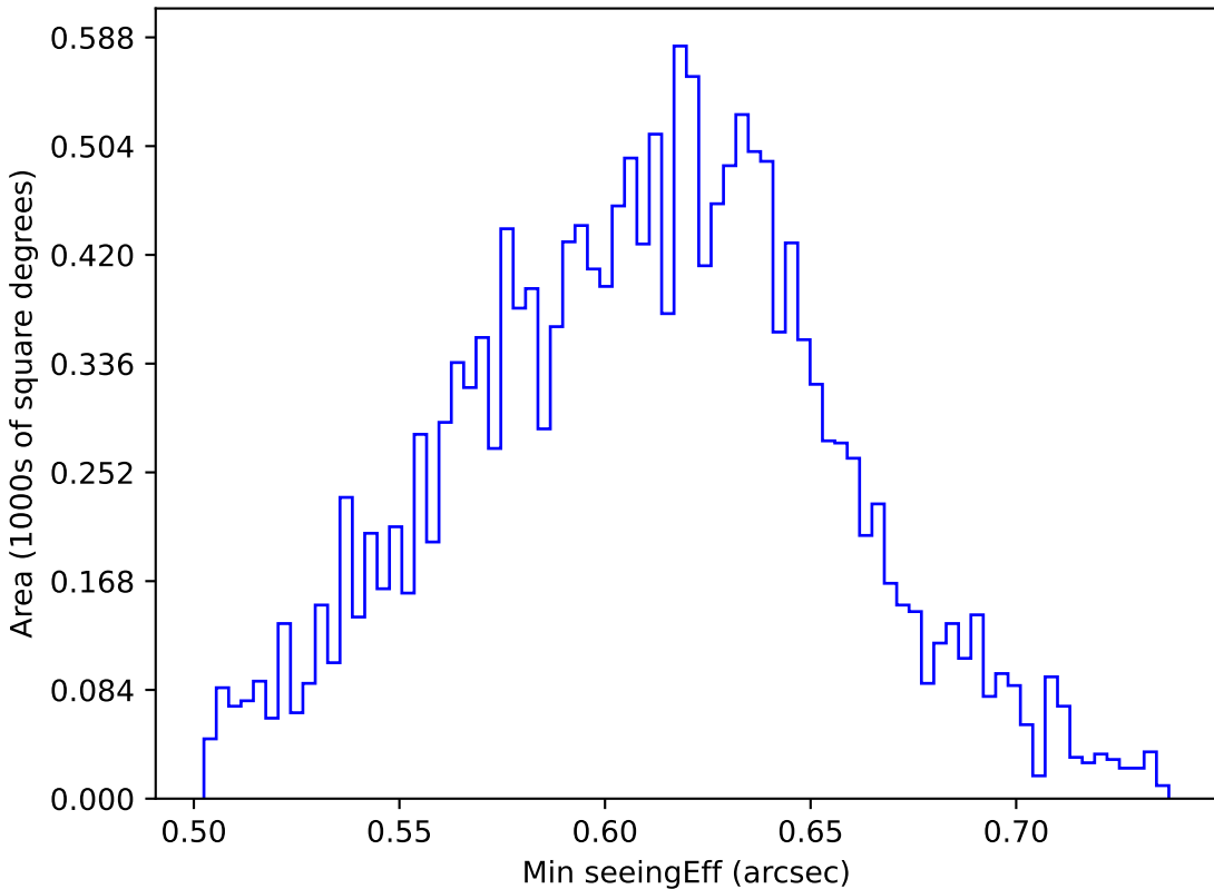
early_u_fpextra3.0_v3.4_10yrs WFD r band: Min seeingEff
