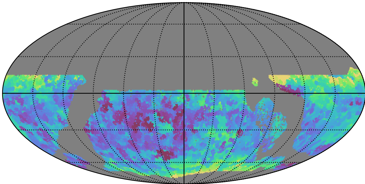
early_u_fpextra3.0_v3.4_10yrs WFD i band: Min seeingEff
