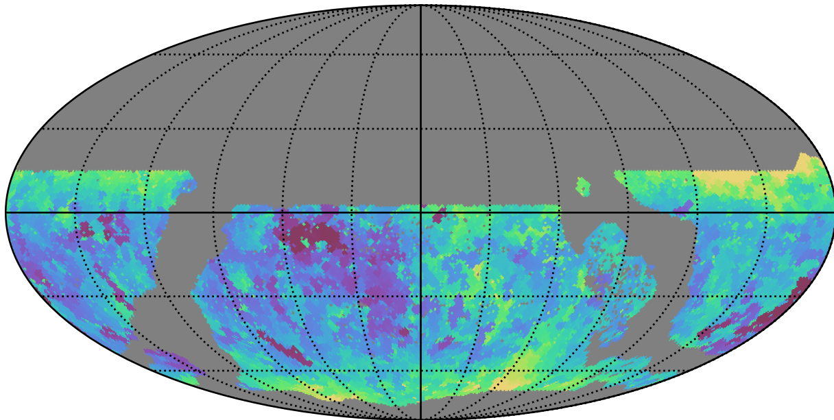
early_u_fpextra3.0_v3.4_10yrs WFD g band: Min seeingEff
