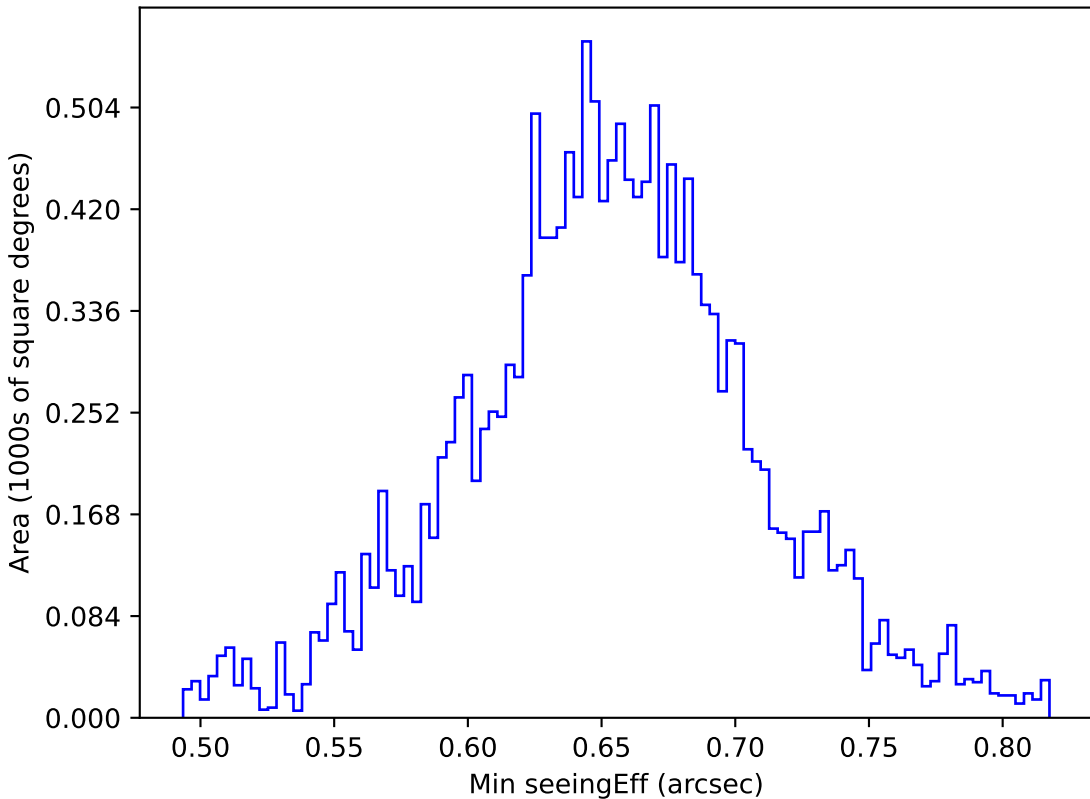
early_u_fpextra3.0_v3.4_10yrs WFD g band: Min seeingEff
