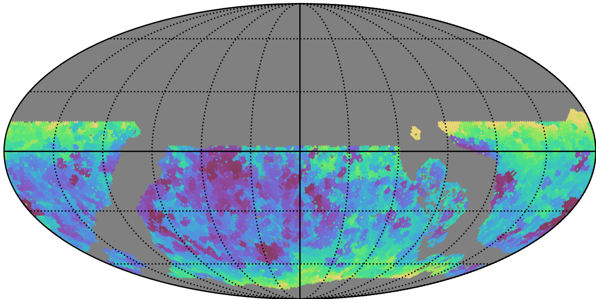
early_u_fpextra3.0_v3.4_10yrs WFD all bands: Min seeingEff
