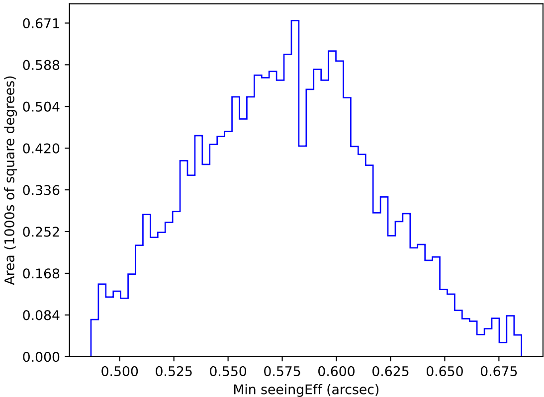
early_u_fpextra3.0_v3.4_10yrs WFD all bands: Min seeingEff
