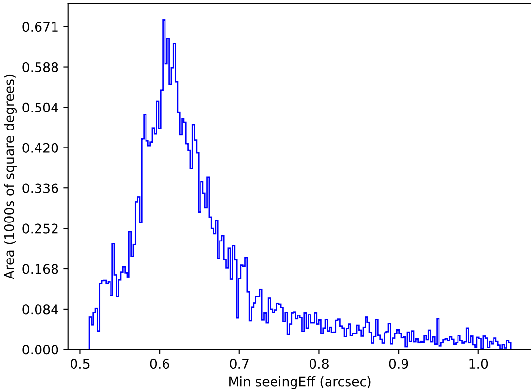
early_u_fpextra3.0_v3.4_10yrs All sky z band: Min seeingEff
