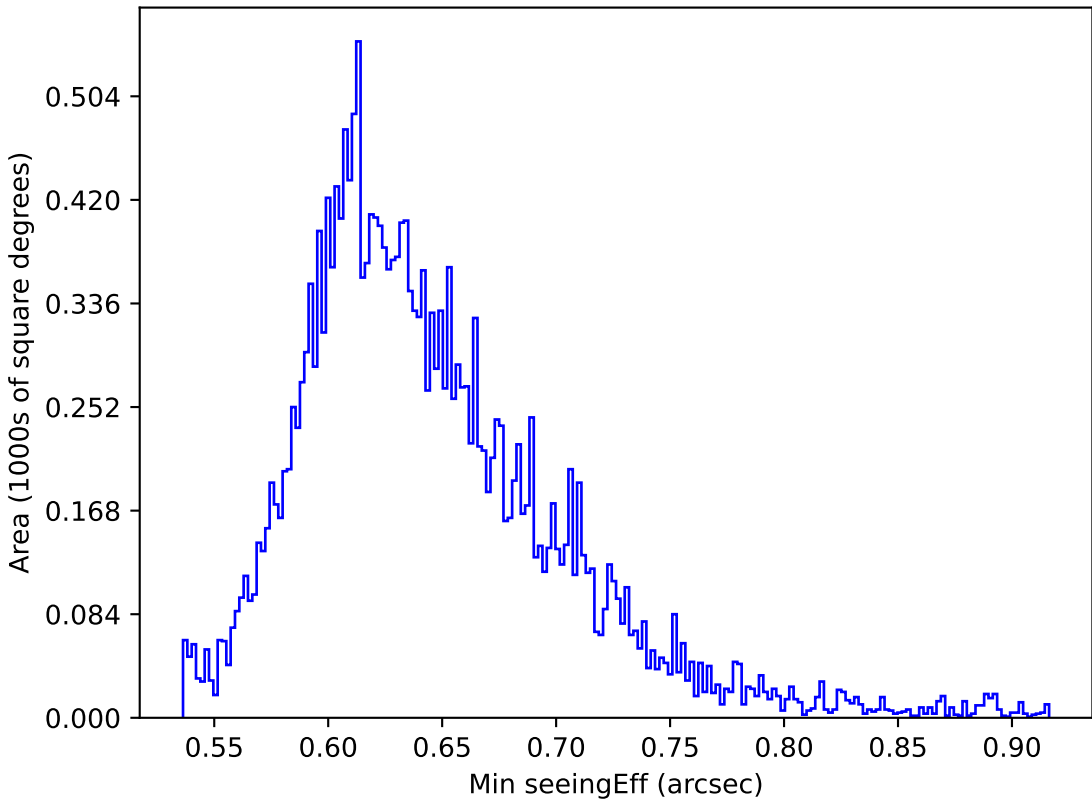
early_u_fpextra3.0_v3.4_10yrs All sky y band: Min seeingEff
