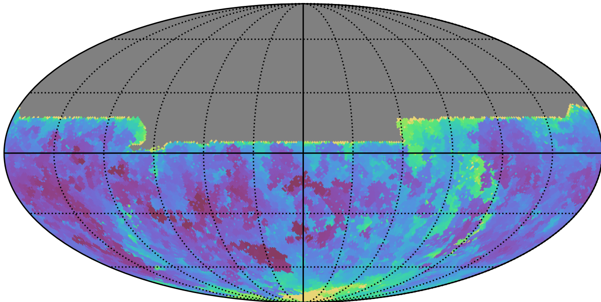
early_u_fpextra3.0_v3.4_10yrs All sky u band: Min seeingEff
