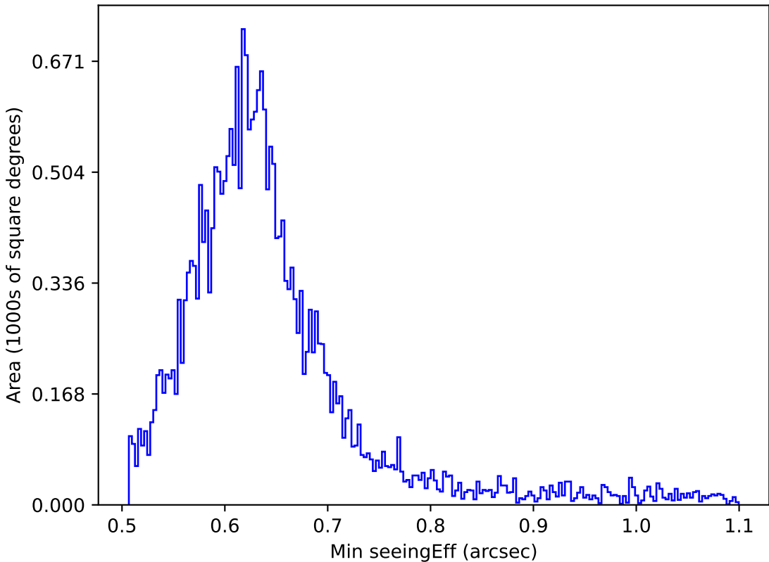
early_u_fpextra3.0_v3.4_10yrs All sky r band: Min seeingEff
