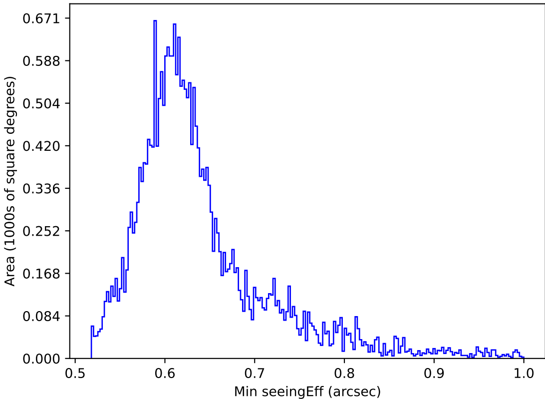
early_u_fpextra3.0_v3.4_10yrs All sky i band: Min seeingEff
