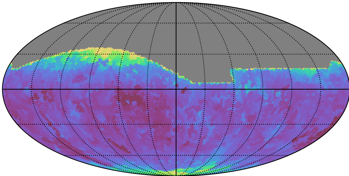
early_u_fpextra3.0_v3.4_10yrs All sky g band: Min seeingEff
