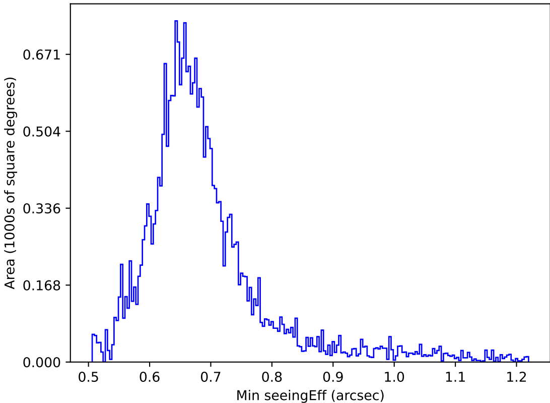
early_u_fpextra3.0_v3.4_10yrs All sky g band: Min seeingEff
