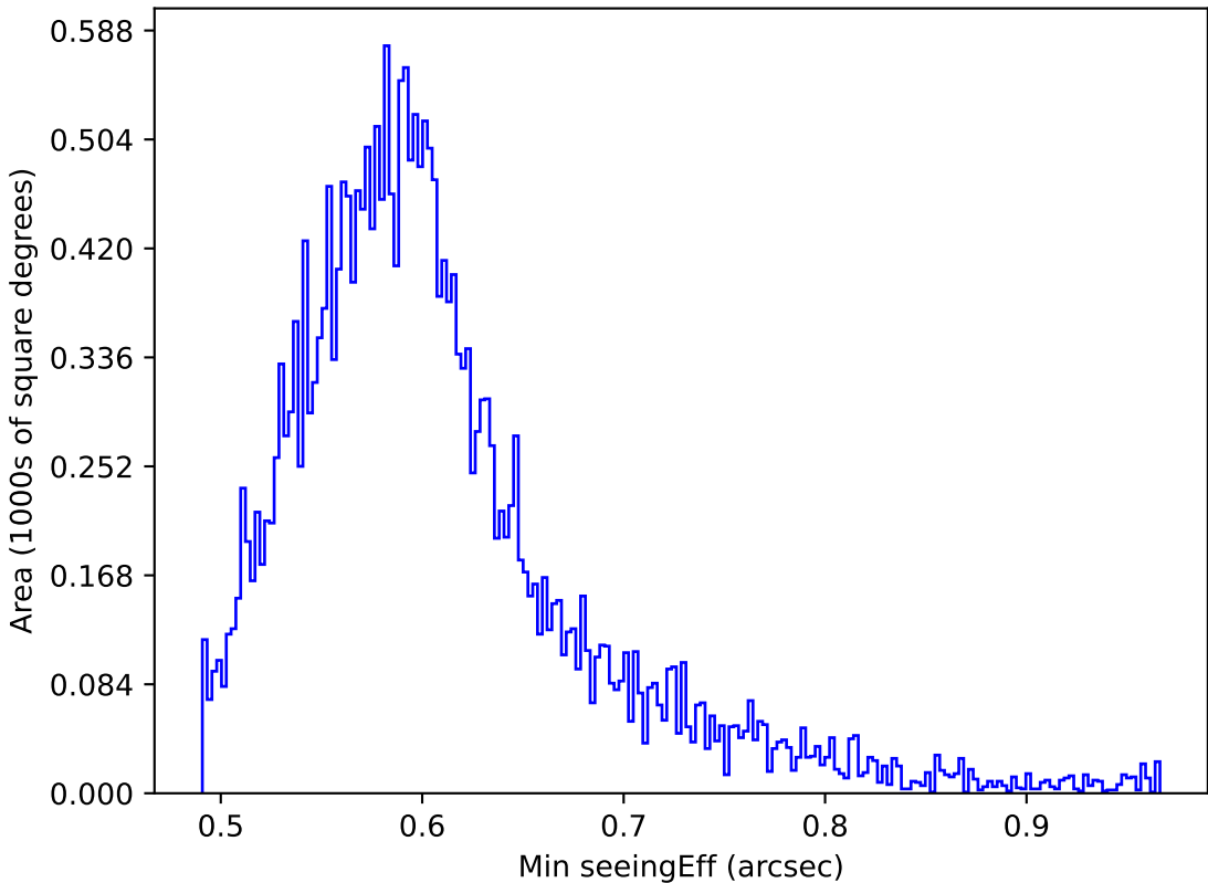
early_u_fpextra3.0_v3.4_10yrs All sky all bands: Min seeingEff
